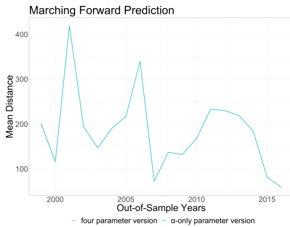
Figure 2. Mean Haversine Distance between Forecast and Observed locations.
