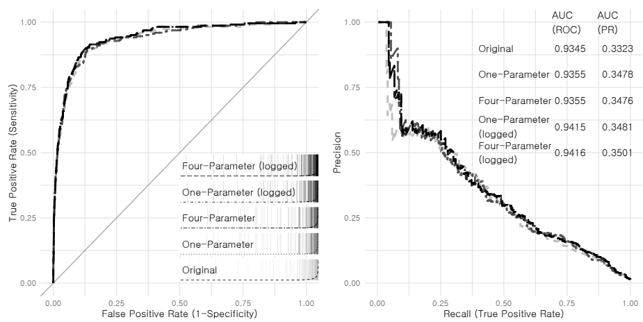
Figure 6. Out-of-sample predictive performance
