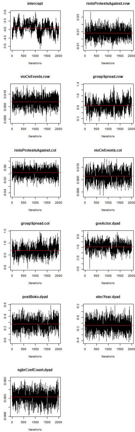
Figure 7. Traceplots with 50,000 iterations
